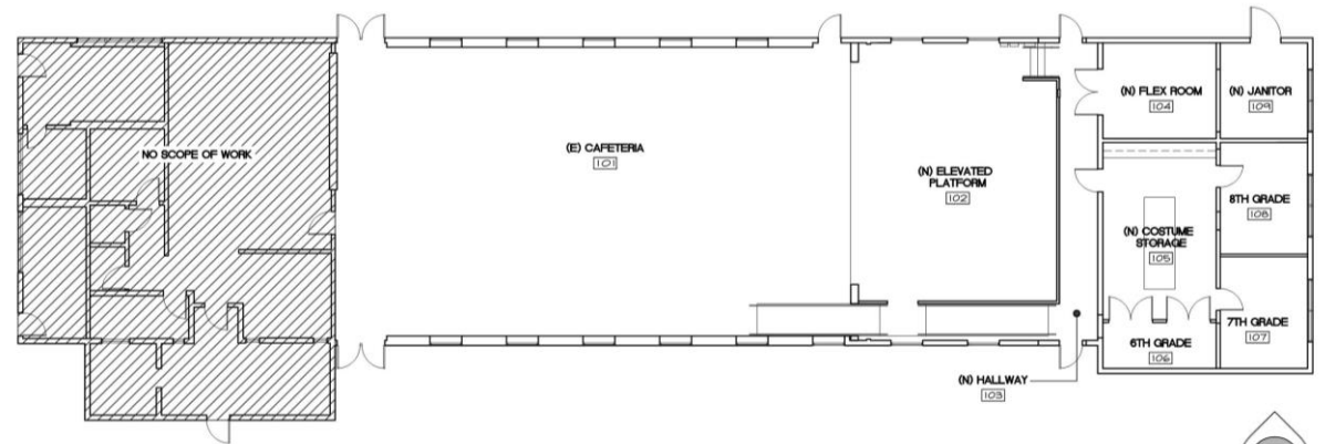
FLOOR PLAN
